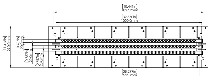
POSSIBLE TOP DUCT CONNECTION
