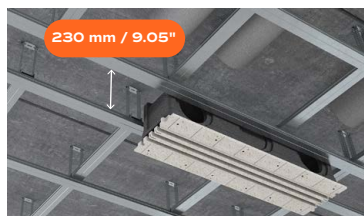
Minimum installation height: 230 mm / 9.05"
